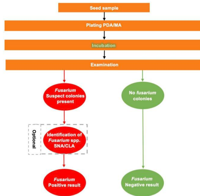
Figure 1. Workflow describing the steps and decisions for detection of Fusarium spp. by plating on media and morphological identification.
